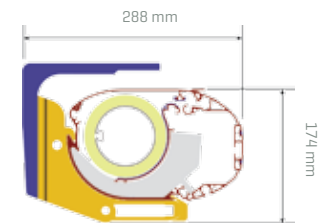
Fitting to the ceiling ceiling bows*
