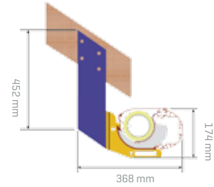
Fitting to the trusses roof trusses*
