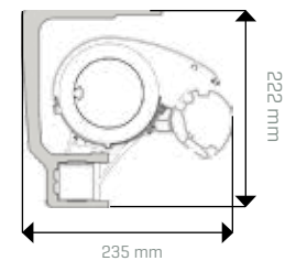
Fitting to the ceiling ceiling consoles*
