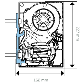
Fitting to the wall wall brackets
