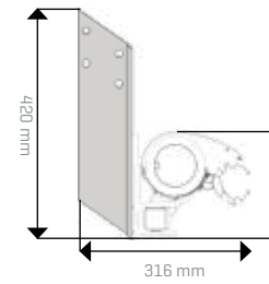
Fitting to the trusses roof trusses*
